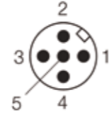
M12 connector
